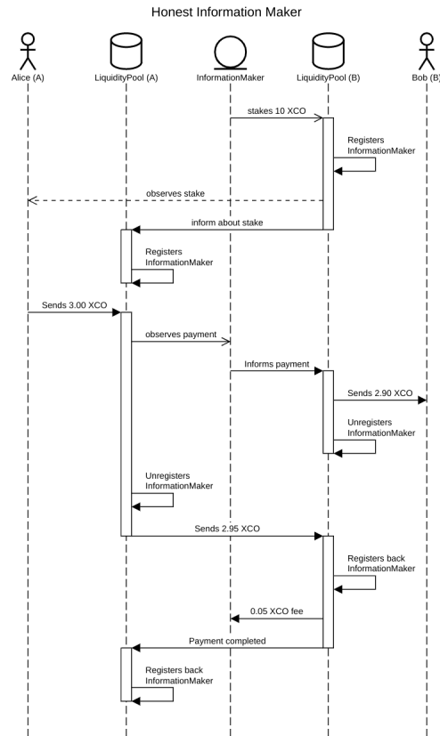
Figure 7: Information market maker example: Alice sends XCO stored on blockchain A, to Bob on blockchain B. To expedite the process and avoid the long delay between blockchains A and B, Alice uses an information market maker.
