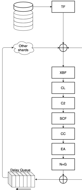
Figure 10: Execution pipeline
